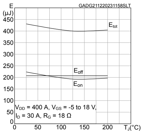
Figure 11. Typical switching energy vs temperature
