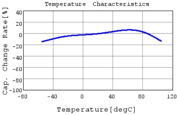
GRM033C80J104ME15 C-Temp. capchange, DC0.0V,
