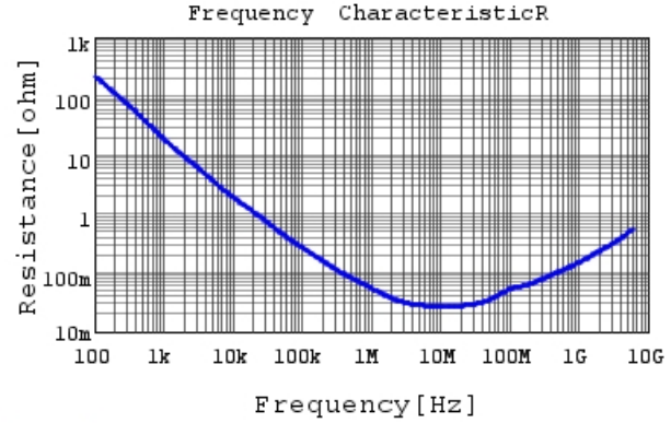
GRM033C80J104ME15 R DCOV, 25degC
