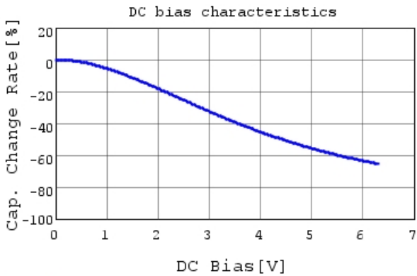
GRM033C80J104ME15 C-DC bias capchange, 25.0c
