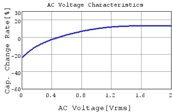
GRM033C80J104ME15 C-AC Voltage capchange, Dc
