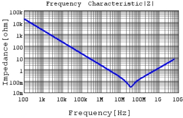
GRM033C80J104ME15 |Z| DCOV, 25degC
