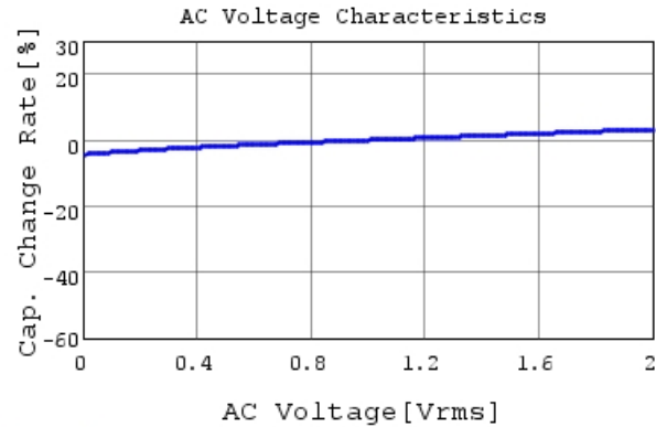
GRM033R71A152KA01 C-AC Voltage capchange, Dc
