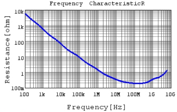
GRM033R71A152KA01 R DCOV, 25degC
