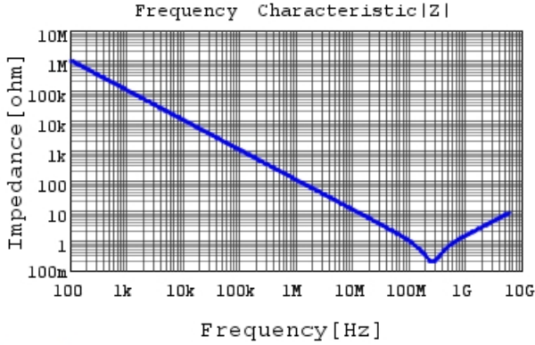
GRM033R71A152KA01 |Z| DCOV, 25degC
