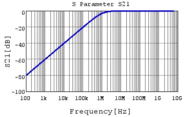
GRM033R71A152KA01 S21 DC0V, 25degC
