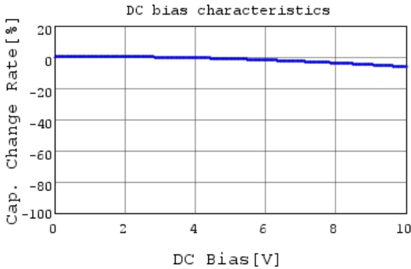
GRM033R71A152KA01 C-DC bias capchange, 25.0c
