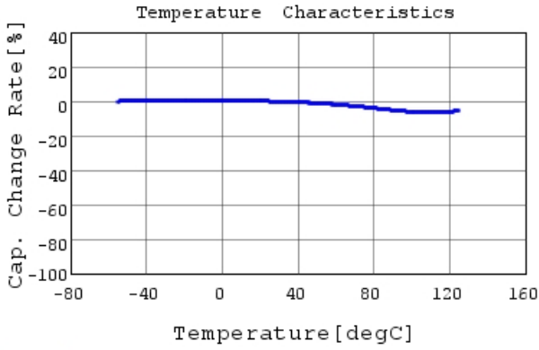
GRM033R71A152KA01 C-Temp. capchange, DC0.0V,
