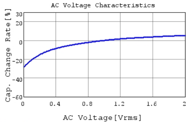
GRM033Z71C104ME14 C-AC Voltage capchange, Dc
