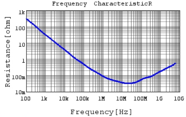
GRM033Z71C104ME14 R DCOV,25degC
