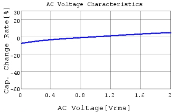
GRM033C81E103KE14 C-AC Voltage capchange, Dc
