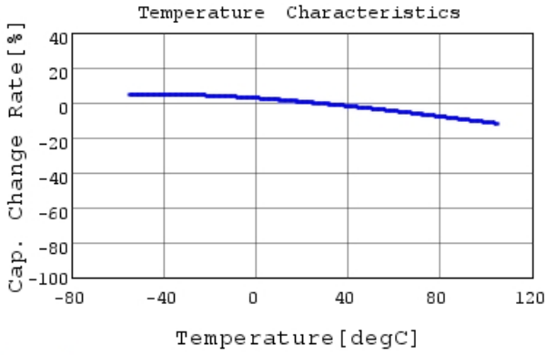
GRM033C81E103KE14 C-Temp. capchange, DC0.0V,
