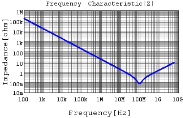
GRM033C81E103KE14 |Z| DCOV, 25degC
