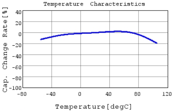
GRM035C80J225ME01 C-Temp. capchange, DC0.0V,
