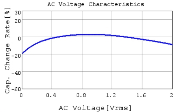
GRM035C80J225ME01 C-AC Voltage capchange, Dc
