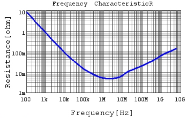
GRM035C80J225ME01 R DCOV, 25degC
