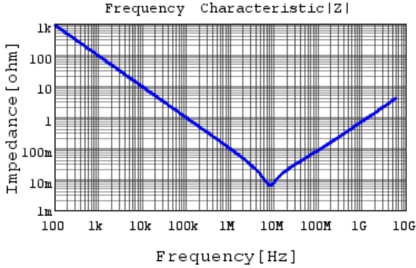
GRM035C80J225ME01 |Z| DCOV, 25degC
