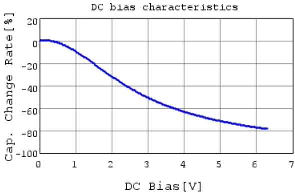
GRM035C80J225ME01 C-DC bias capchange, 25.0c
