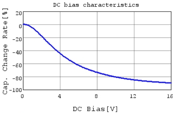
GRM033R61C104ME18 C-DC bias capchange, 25.0c
