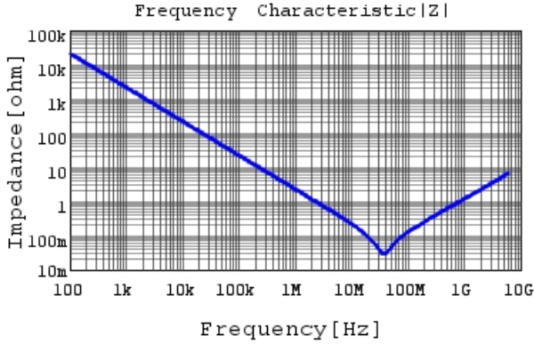
GRM033R61C104ME18 |Z| DCOV,25degC
