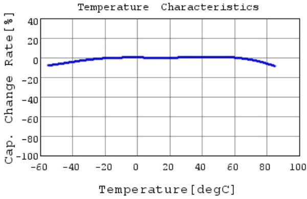
GRM033R61C104ME18 C-Temp. capchange, DCO.OV,
