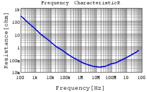
GRM033R61C104ME18 R DCOV,25degC
