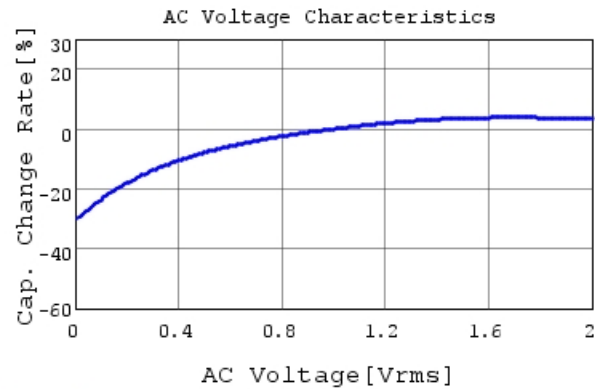
GRM033R61C104ME18 C-AC Voltage capchange, Dc
