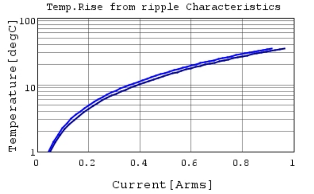
GRM033R61C104ME18 Temp.rise 800kHz
