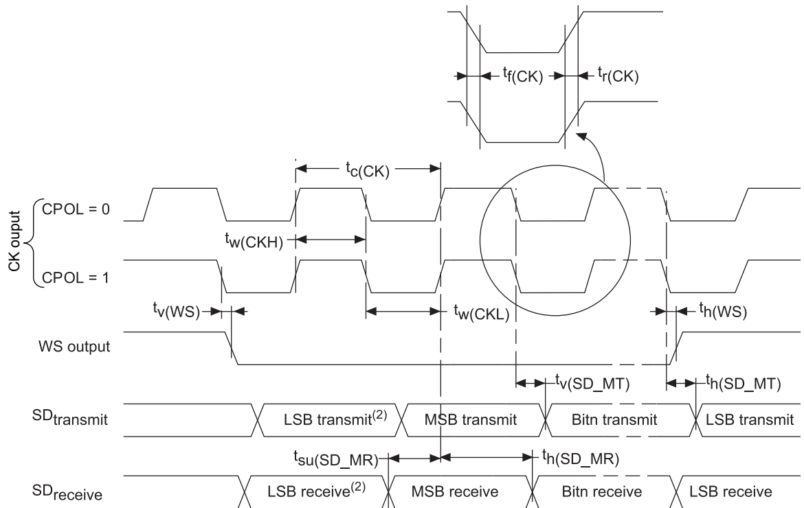
Figure 51. I2S master timing diagram (Philips protocol)
