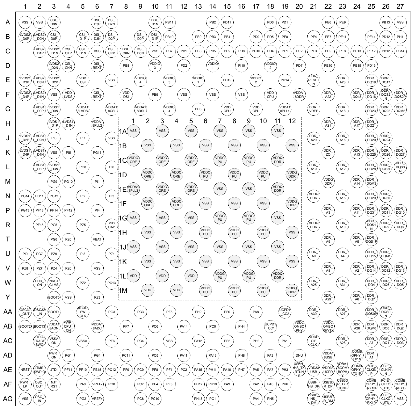
Figure 7. STM32MP25xC/F VFBGA424 pinout
