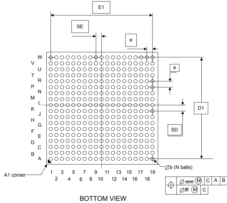
Figure 64. VFBGA361 - Outline
