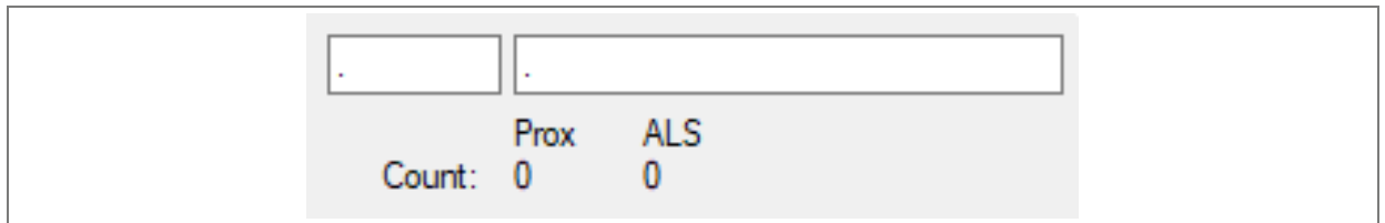
Figure 9: Logging status
