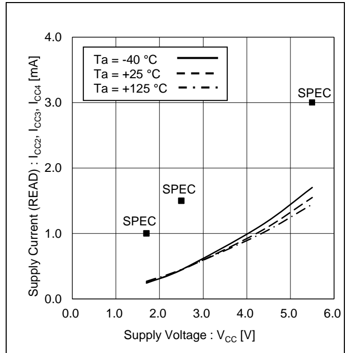
Figure 16. Supply Current (READ) vs Supply Voltage
