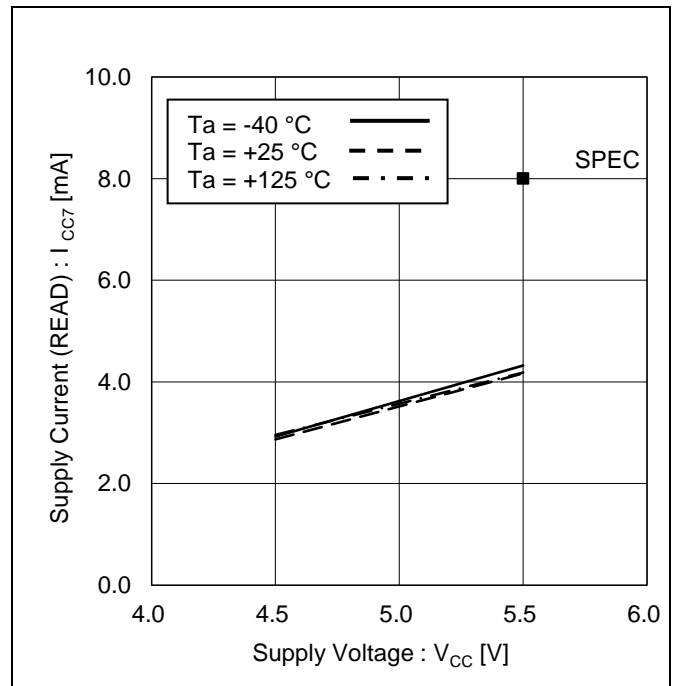
Figure 18. Supply Current (READ) vs Supply Voltage
