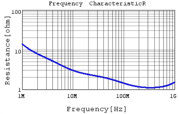
DK1B3EA331K86RBH01 R DCOV, 20degC
