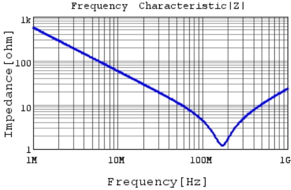
DK1B3EA331K86RBH01 |Z| DCOV, 20degC
