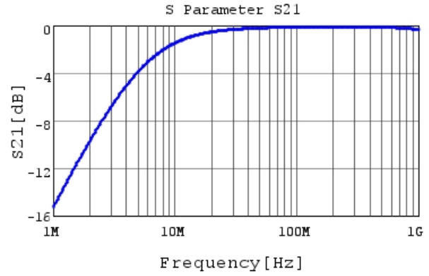
DK1B3EA331K86RBH01 S21 DCOV, 20degC
