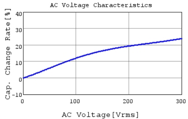
DK1B3EA331K86RBH01 C-AC Voltage capchange, I
