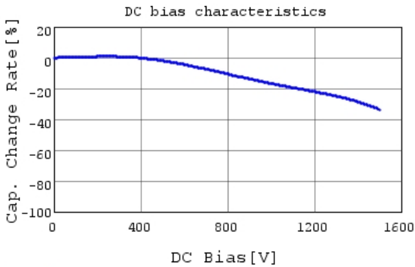
DK1B3EA331K86RBH01 C-DC bias capchange, 20.0
