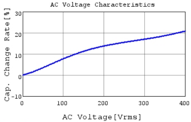
DE1B3RA101KA4BH01F C-AC Voltage capchange, I
