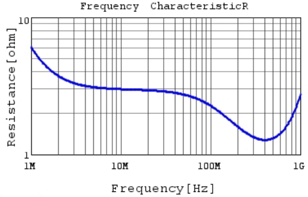
DE1B3RA101KA4BH01F R DCOV, 20degC
