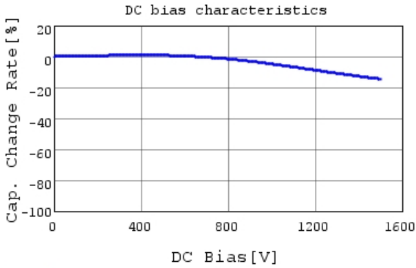
DE1B3RA101KA4BH01F C-DC bias capchange, 20.0
