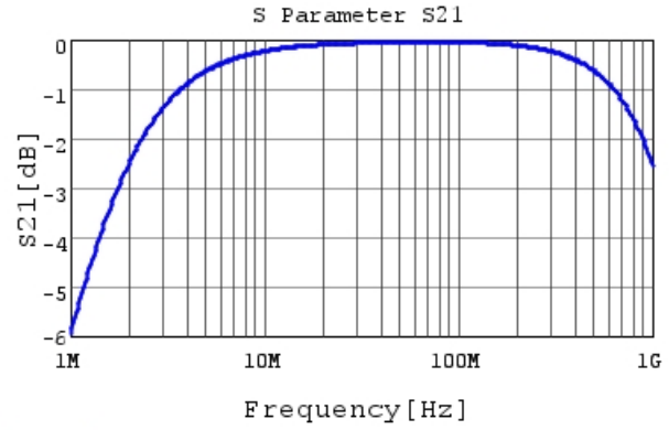
DE1E3RA102MN4AP01F S21 DCOV, 20degC
