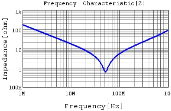
DE1E3RA102MN4AP01F |Z| DCOV, 20degC
