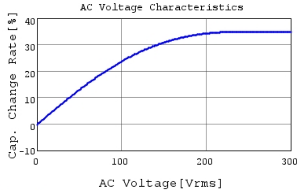
DE1E3RA102MN4AP01F C-AC Voltage capchange, I
