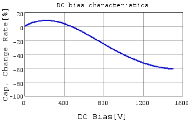
DE1E3RA472MN4AH01F C-DC bias capchange, 20.0
