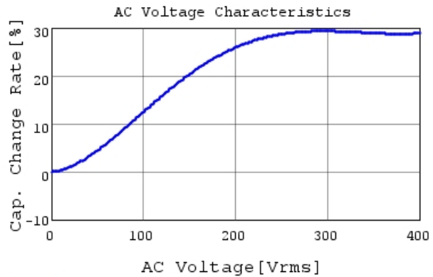
DE1E3RA472MN4AH01F C-AC Voltage capchange, I
