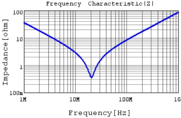
DE1E3RA472MN4AH01F |Z| DCOV, 20degC
