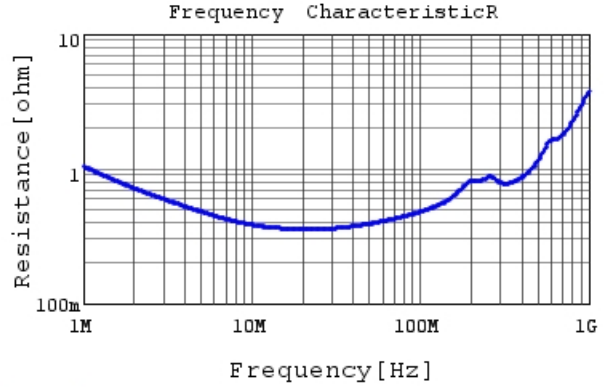
DE1E3RA472MN4AH01F R DCOV, 20degC
