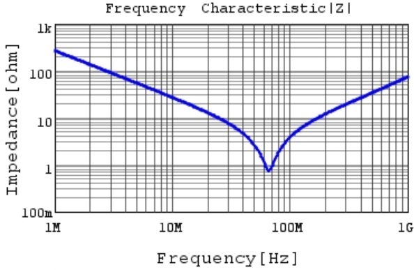
DE2B3SA681KA3BY02F |Z| DCOV, 20degC
