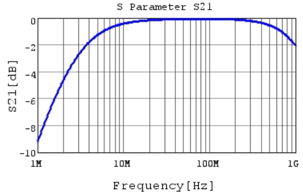
DE2B3SA681KA3BY02F S21 DCOV, 20degC
