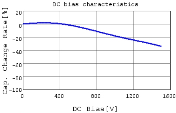
DE2B3SA681KA3BY02F C-DC bias capchange, 20.0
