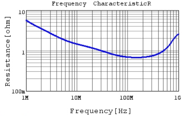
DE2B3SA681KA3BY02F R DCOV, 20degC
