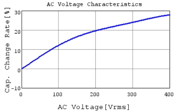
DE2B3SA681KA3BY02F C-AC Voltage capchange, I
