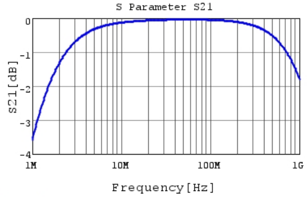
DE2E3SA152MA3BY02F S21 DCOV, 20degC
