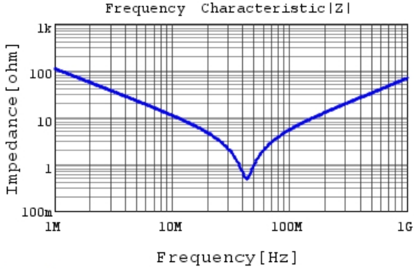
DE2E3SA152MA3BY02F |Z| DCOV, 20degC
