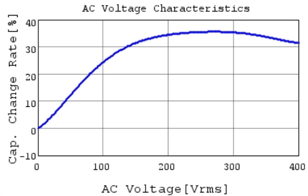
DE2E3SA152MA3BY02F C-AC Voltage capchange, I
