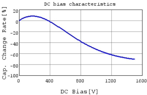
DE2E3SA152MA3BY02F C-DC bias capchange, 20.0
