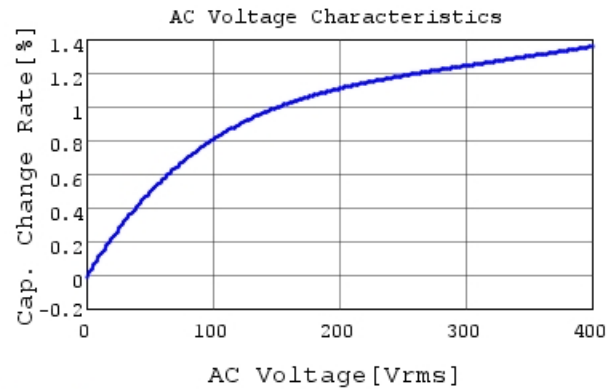
DE11XRA100KJ4BH01F C-AC Voltage capchange, I
