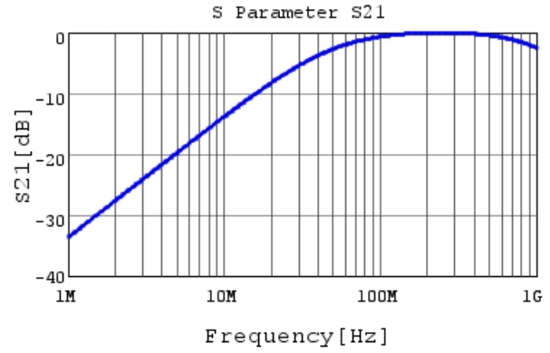
DE11XRA330KA4BH01F S21 DCOV, 20degC
