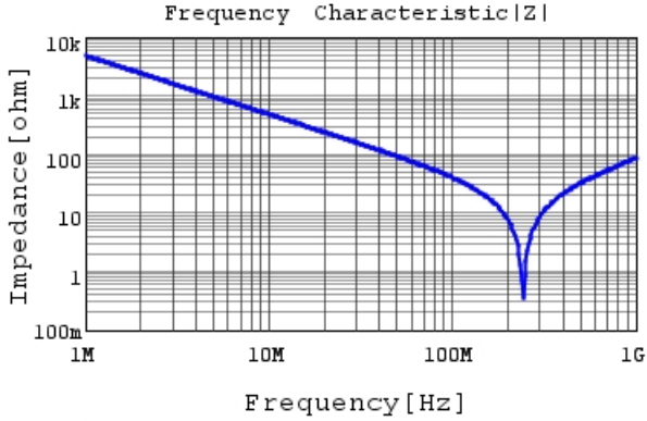
DE11XRA330KJ4BH01F |Z| DC0V, 20degC
