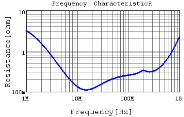
DE11XRA680KA4BH01F R DC0V, 20degC
