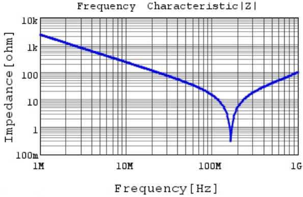
DE11XRA680KA4BH01F |Z| DC0V, 20degC
