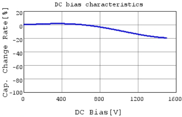
DE1B3RA151KA4BH01F C-DC bias capchange, 20.0
