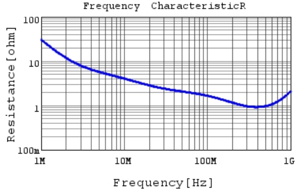
DE1B3RA151KA4BH01F R DCOV, 20degC
