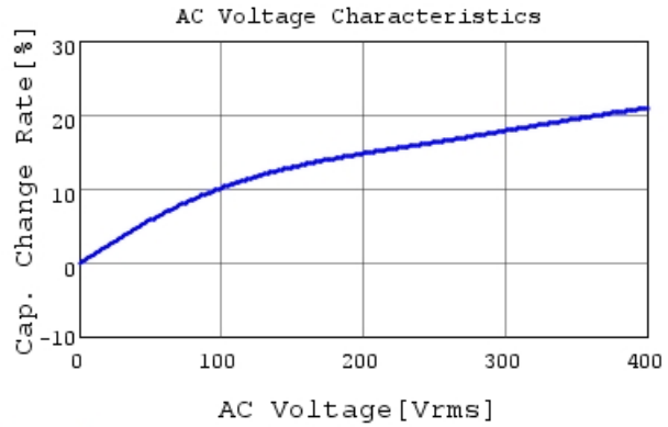
DE1B3RA151KA4BH01F C-AC Voltage capchange, I
