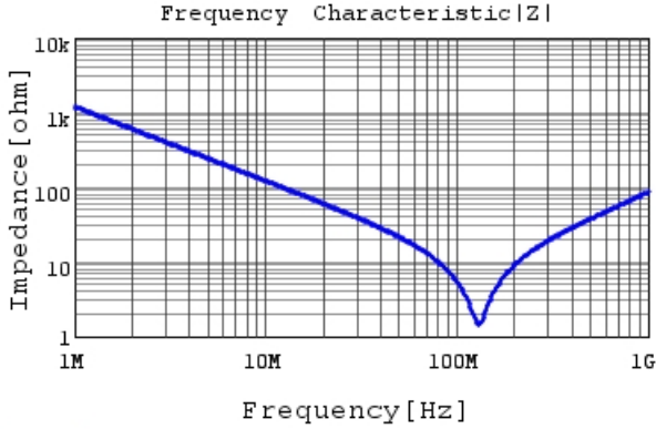
DE1B3RA151KA4BH01F |Z| DCOV, 20degC
