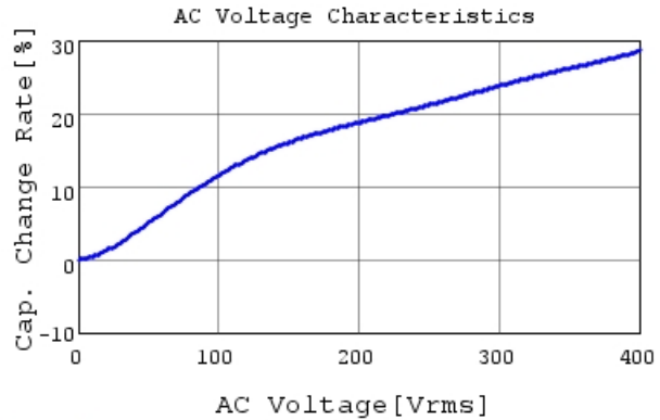
DE1B3RA221KA4BH01F C-AC Voltage capchange, I
