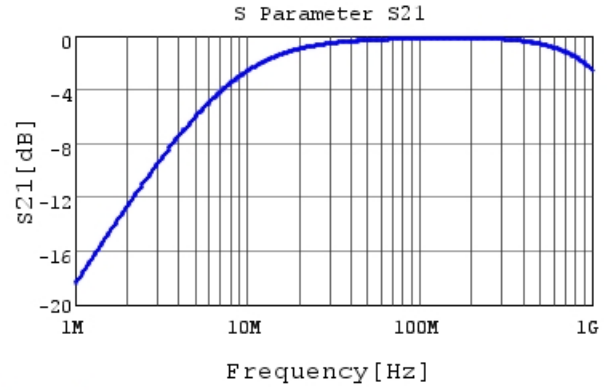
DE1B3RA221KA4BH01F S21 DCOV, 20degC
