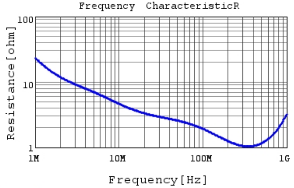
DE1B3RA221KA4BH01F R DCOV, 20degC
