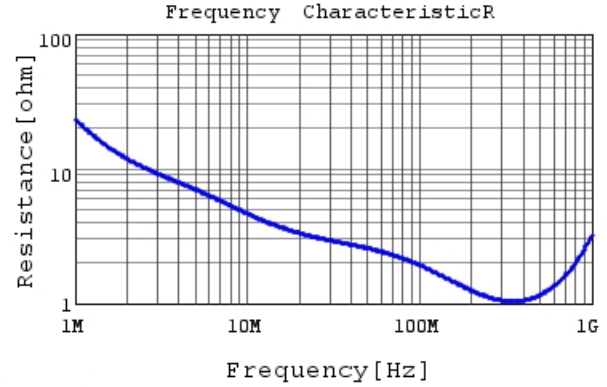
DE1B3RA221KN4AH01F R DCOV, 20degC
