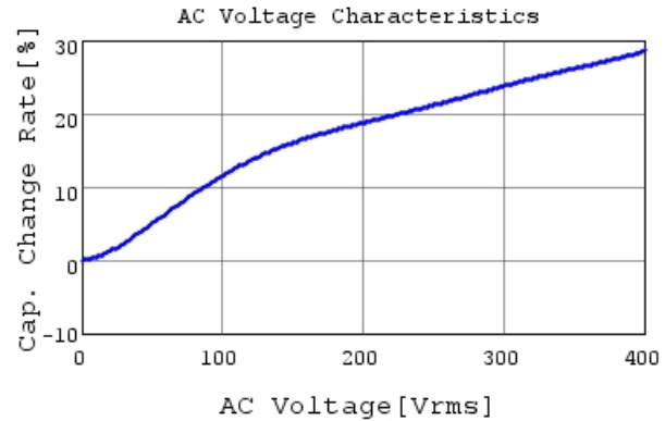
DE1B3RA221KN4AH01F C-AC Voltage capchange, I
