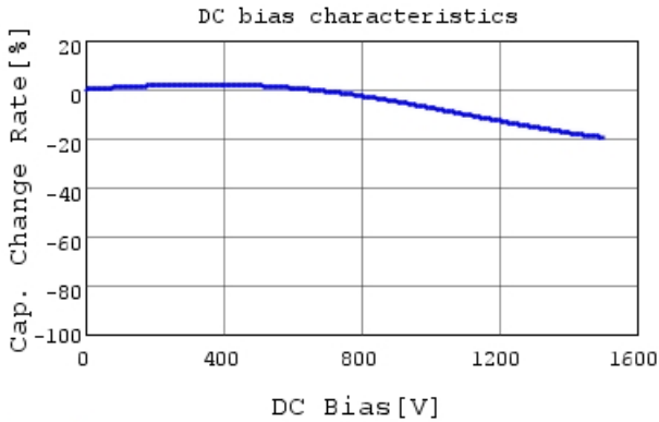
DE1B3RA221KN4AH01F C-DC bias capchange, 20.0
