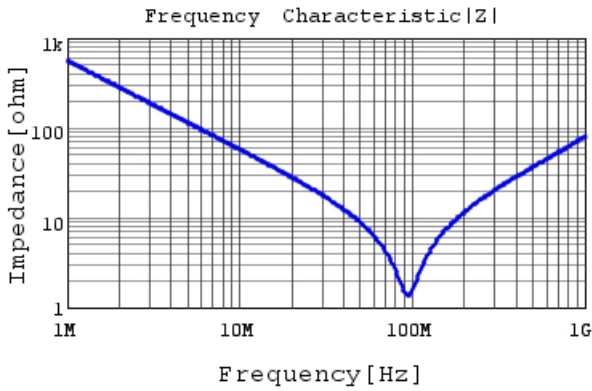
DE1B3RA331KA4BH01F |Z| DCOV, 20degC
