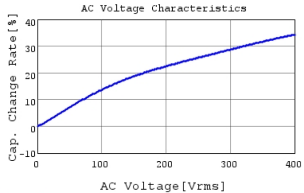
DE1B3RA331KA4BH01F C-AC Voltage capchange, I
