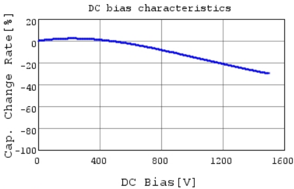
DE1B3RA331KA4BH01F C-DC bias capchange, 20.0
