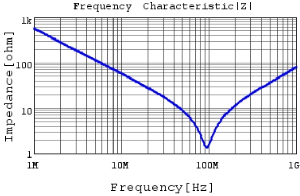
DE1B3RA331KN4AH01F |Z| DCOV, 20degC
