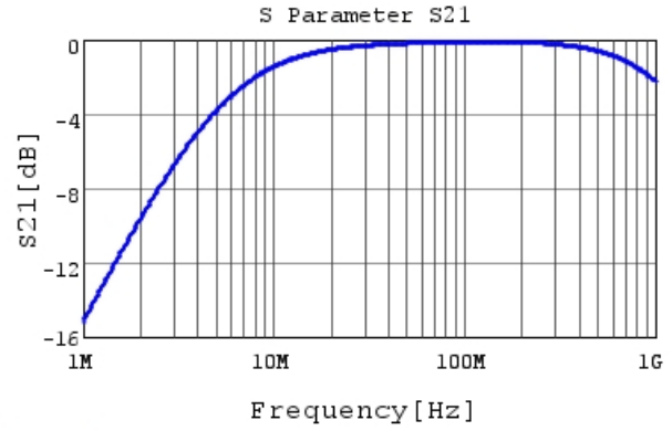
DE1B3RA331KN4AH01F S21 DCOV, 20degC
