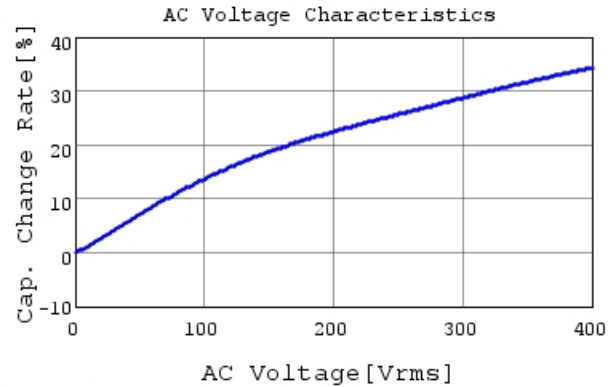
DE1B3RA331KN4AH01F C-AC Voltage capchange, I
