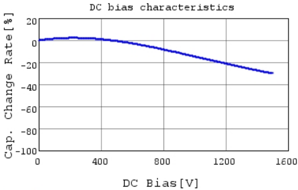
DE1B3RA331KN4AH01F C-DC bias capchange, 20.0
