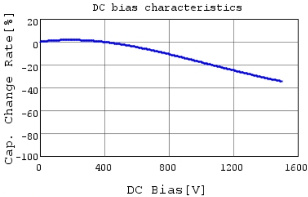
DE1B3RA471KA4BH01F C-DC bias capchange, 20.0
