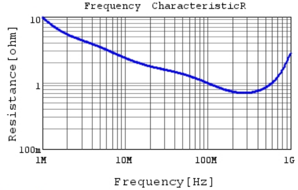
DE1B3RA471KA4BH01F R DC0V, 20degC
