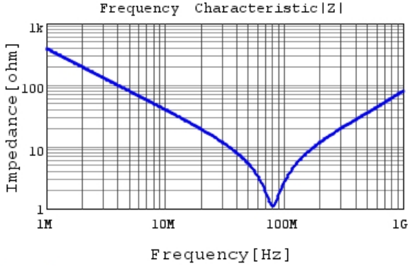
DE1B3RA471KA4BH01F |Z| DC0V, 20degC
