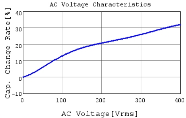
DE1B3RA471KA4BH01F C-AC Voltage capchange, I
