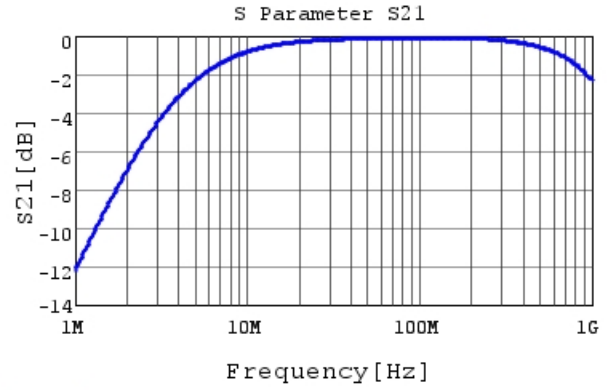
DE1B3RA471KA4BH01F S21 DCOV, 20degC
