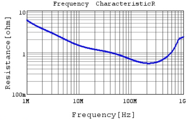
DE1B3RA681KA4BH01F R DCOV, 20degC
