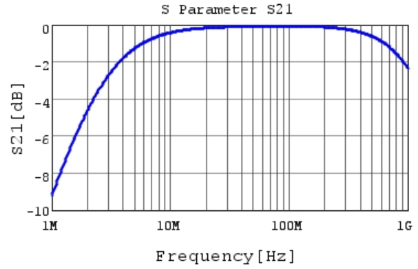
DE1B3RA681KA4BH01F S21 DCOV, 20degC
