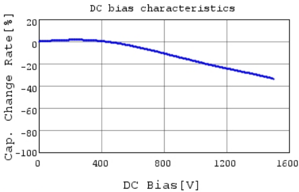
DE1B3RA681KA4BH01F C-DC bias capchange, 20.0
