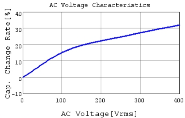
DE1B3RA681KA4BH01F C-AC Voltage capchange, I
