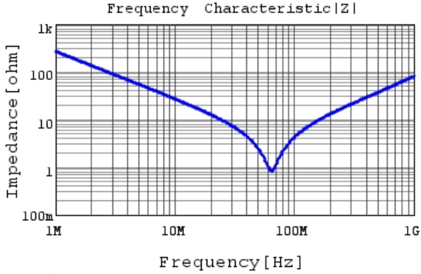
DE1B3RA681KA4BH01F |Z| DCOV, 20degC
