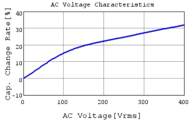
DE1B3RA681KJ4BH01F C-AC Voltage capchange, I
