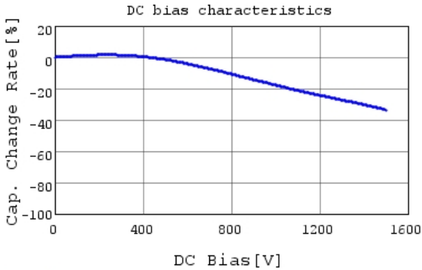
DE1B3RA681KJ4BH01F C-DC bias capchange, 20.0
