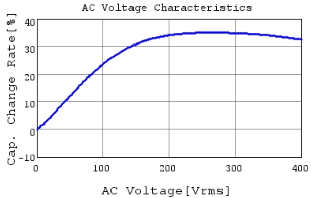
DE1E3RA102MA4BH01F C-AC Voltage capchange, I
