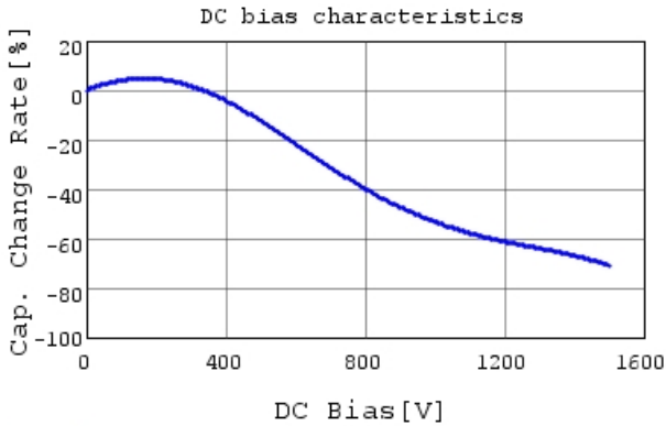
DE1E3RA102MA4BH01F C-DC bias capchange, 20.0
