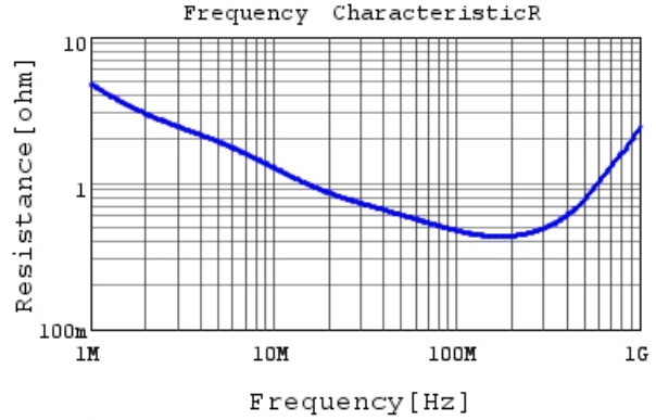
DE1E3RA102MA4BH01F R DCOV, 20degC
