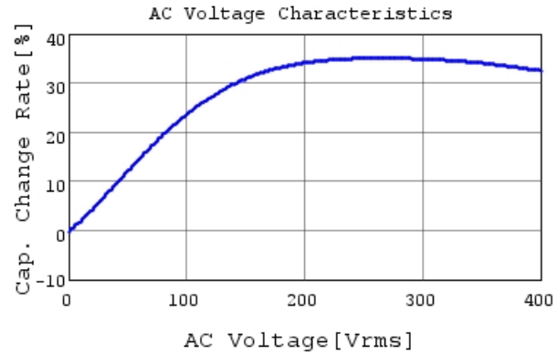
DE1E3RA102MN4AH01F C-AC Voltage capchange, I
