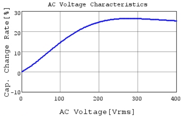
DE1E3RA152MA4BH01F C-AC Voltage capchange, I
