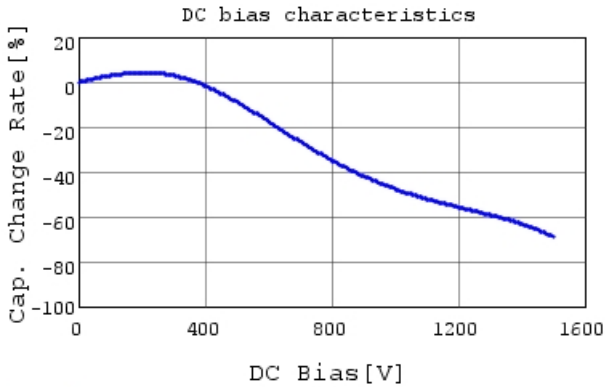
DE1E3RA152MA4BH01F C-DC bias capchange, 20.0
