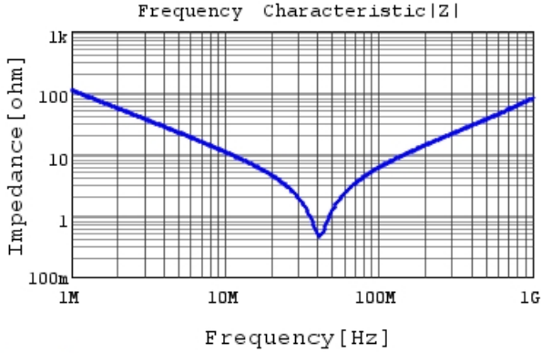
DE1E3RA152MA4BH01F |Z| DCOV, 20degC
