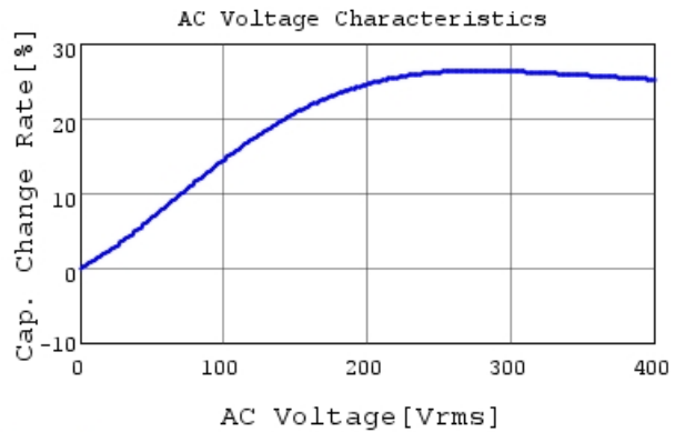
DE1E3RA152MJ4BH01F C-AC Voltage capchange, I
