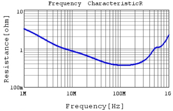
DE1E3RA152MJ4BH01F R DCOV, 20degC
