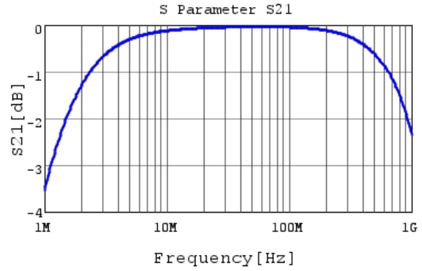
DE1E3RA152MJ4BH01F S21 DCOV, 20degC
