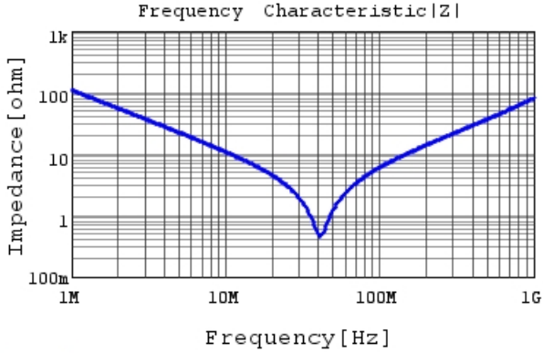
DE1E3RA152MJ4BH01F |Z| DCOV, 20degC
