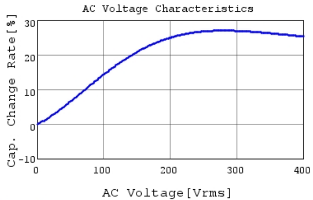
DE1E3RA222MA4BH01F C-AC Voltage capchange, I
