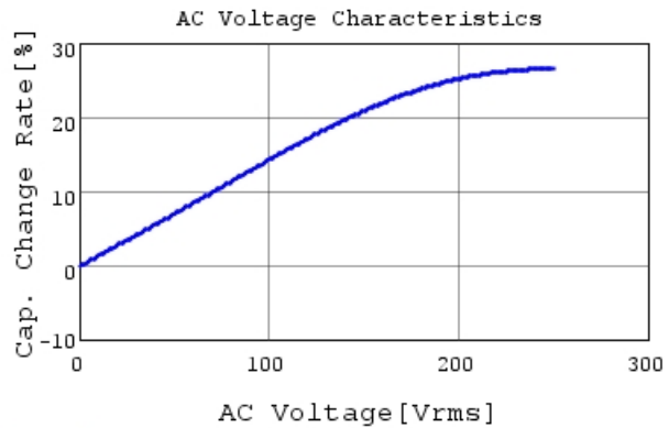
DE1E3RA222MJ4BN01F C-AC Voltage capchange, I
