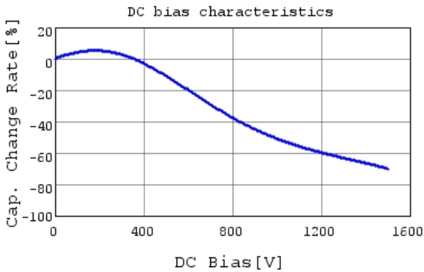
DE1E3RA222MJ4BN01F C-DC bias capchange, 20.0
