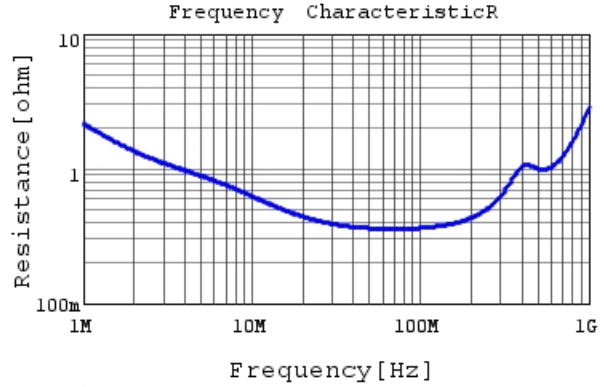
DE1E3RA222MN4AH01F R DCOV, 20degC
