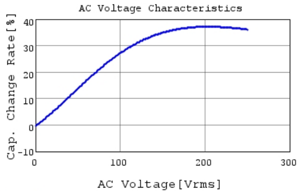
DE2E3SA102MA2BT01F C-AC Voltage capchange, I
