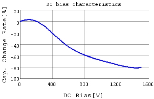
DE2E3SA102MA2BT01F C-DC bias capchange, 20.0
