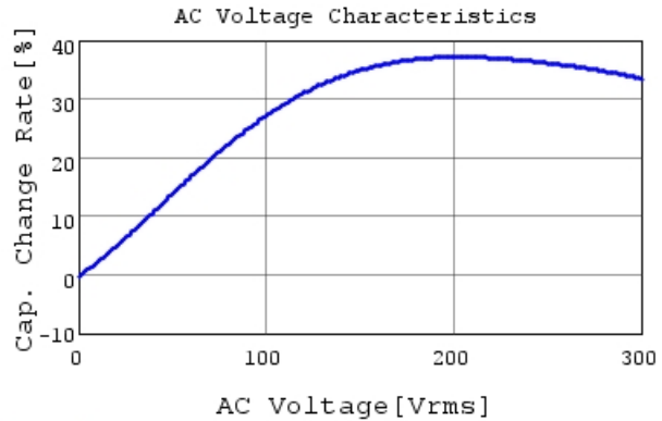
DE2E3SA102MJ3BX02F C-AC Voltage capchange, I
