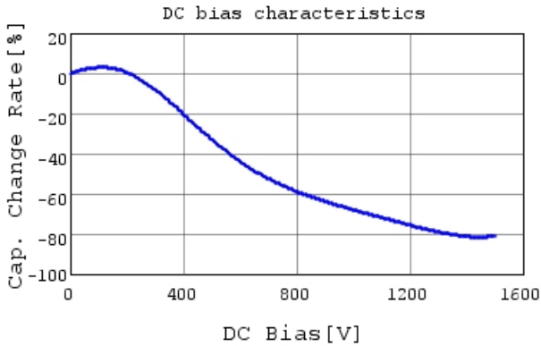
DE2E3SA102MJ3BX02F C-DC bias capchange, 20.0
