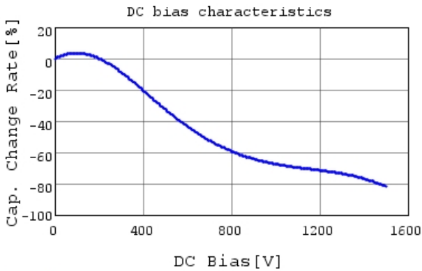
DE2E3SA152MA3BX02F C-DC bias capchange, 20.0
