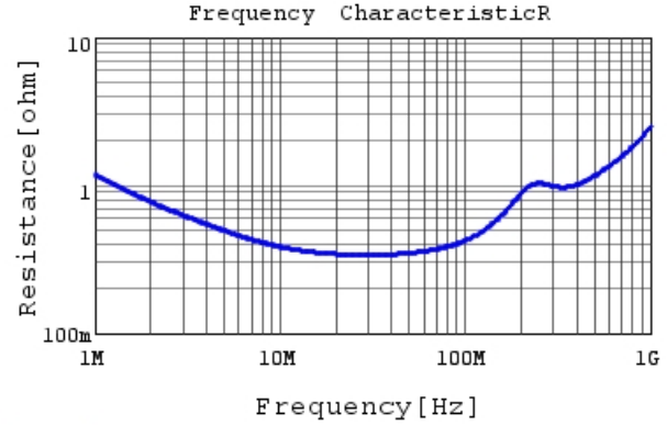
DE2E3SA472MN3AY02F R DCOV, 20degC
