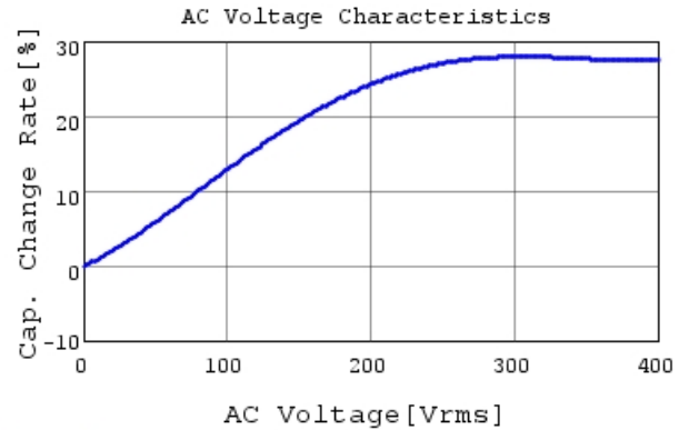
DE2E3SA472MN3AY02F C-AC Voltage capchange, I
