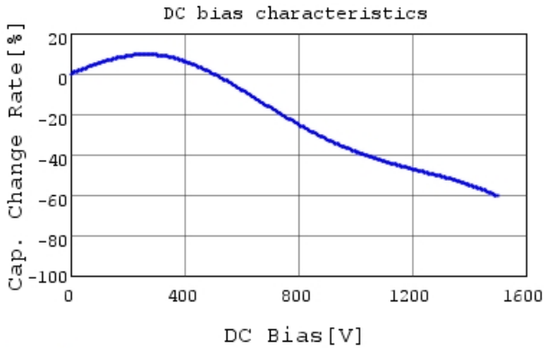
DE2E3SA472MN3AY02F C-DC bias capchange, 20.0
