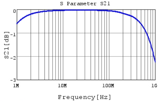
DE2E3SA472MN3AY02F S21 DCOV, 20degC
