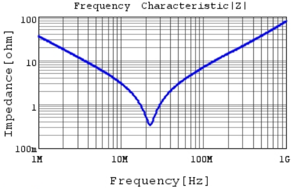
DE2E3SA472MN3AY02F |Z| DCOV, 20degC
