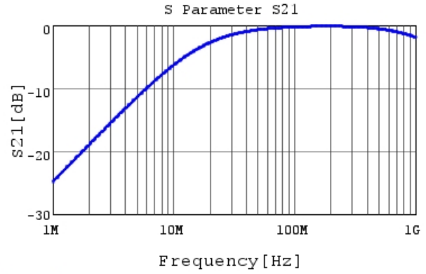
DE6B3KJ101KA3BE01J S21 DCOV, 20degC
