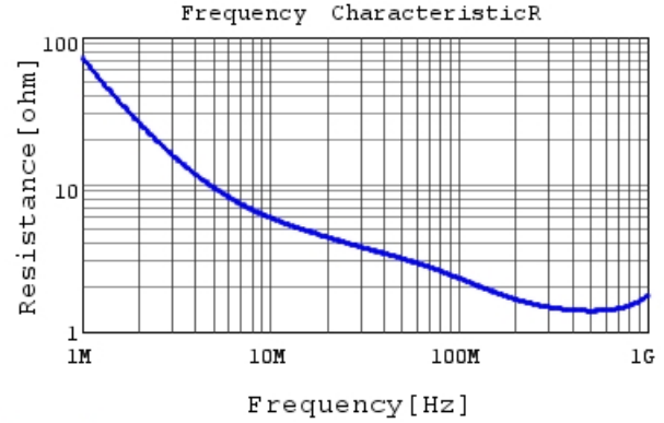
DE6B3KJ101KA3BE01J R DC0V, 20degC
