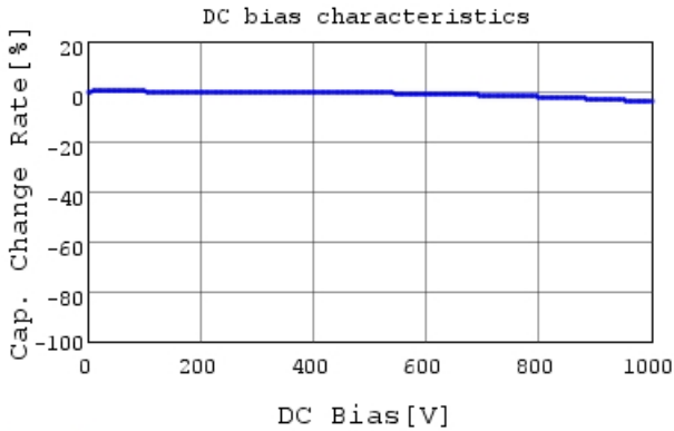
DE6B3KJ101KA4BE01J C-DC bias capchange, 20.0
