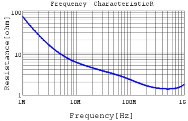
DE6B3KJ101KA4BE01J R DC0V, 20degC
