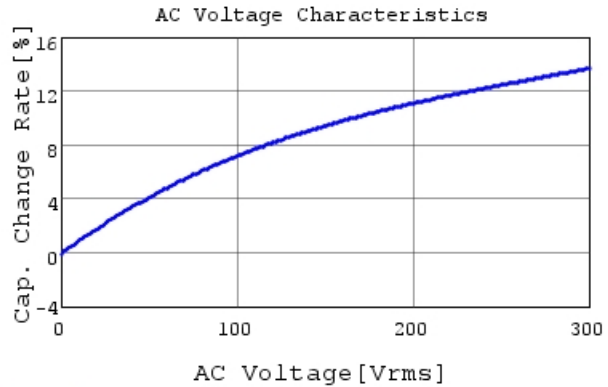
DE6B3KJ101KA4BE01J C-AC Voltage capchange, I
