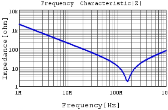
DE6B3KJ101KA4BE01J |Z| DC0V, 20degC
