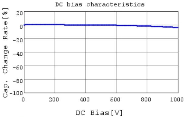
DE6B3KJ151KA3BE01J C-DC bias capchange, 20.0
