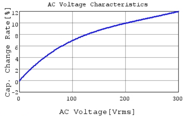
DE6B3KJ151KA3BE01J C-AC Voltage capchange, I
