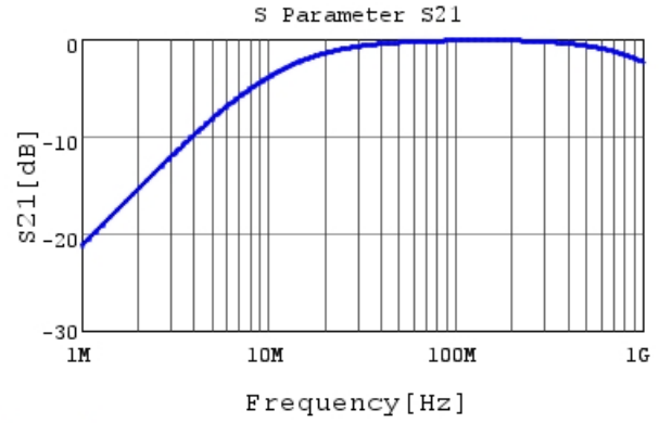
DE6B3KJ151KA3BE01J S21 DCOV, 20degC
