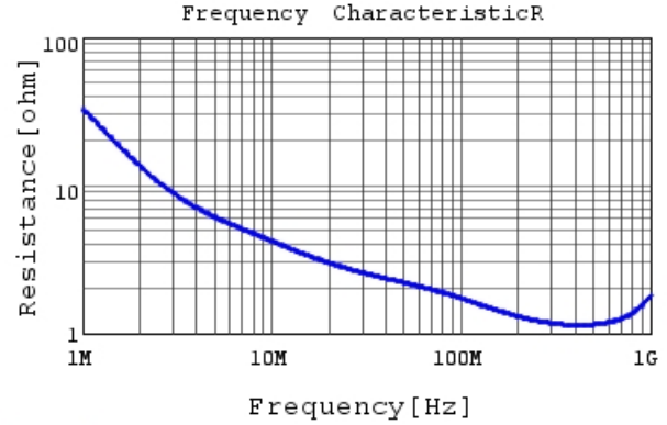
DE6B3KJ151KA3BE01J R DC0V, 20degC
