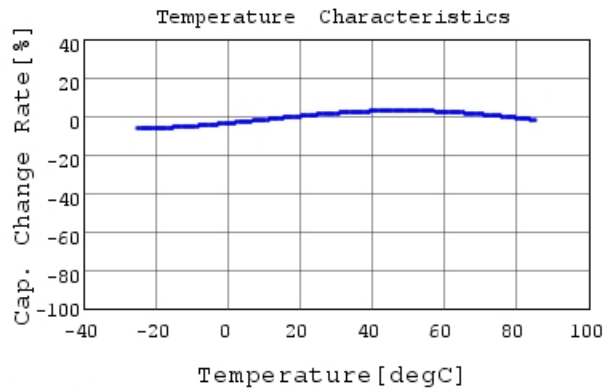
DE6B3KJ151KA4BE01J C-Temp. capchange, DC0V,
