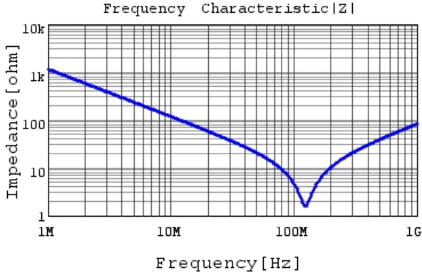
DE6B3KJ151KA4BE01J |Z| DC0V, 20degC
