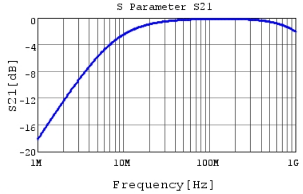
DE6B3KJ221KN4AE01J S21 DCOV, 20degC
