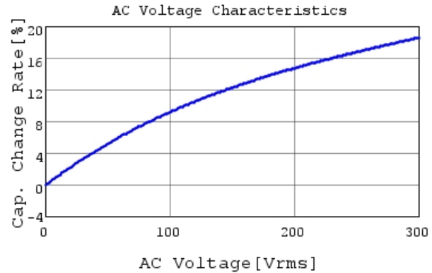
DE6B3KJ221KN4AE01J C-AC Voltage capchange, I
