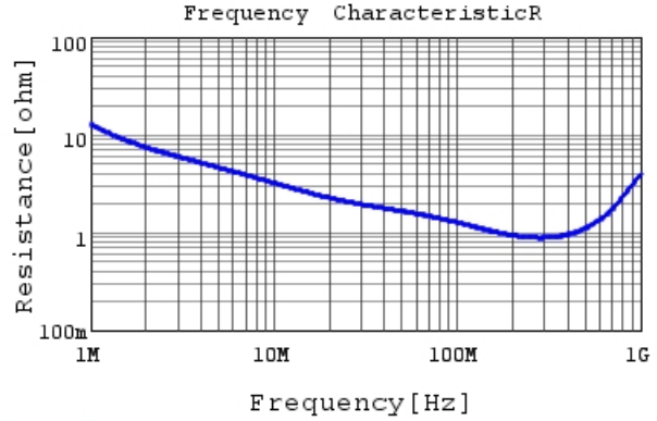
DE6B3KJ331KB4BE01J R DC0V, 20degC
