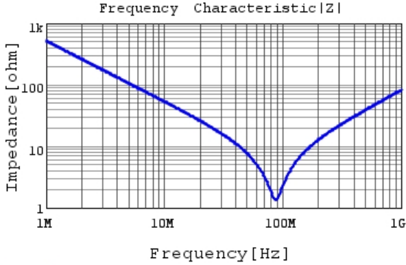
DE6B3KJ331KB4BE01J |Z| DC0V, 20degC
