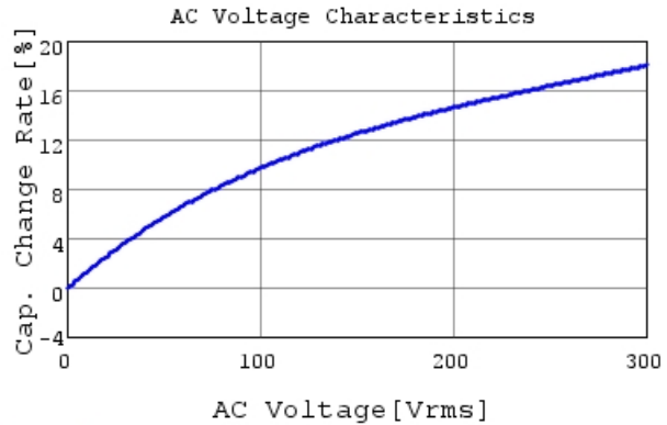
DE6B3KJ331KN4AE01J C-AC Voltage capchange, I
