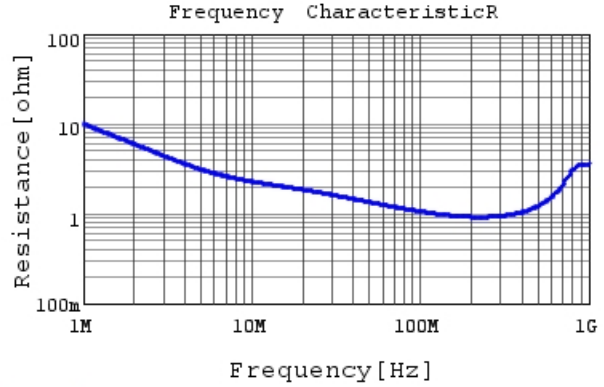
DE6B3KJ471KA3BE01J R DCOV, 20degC
