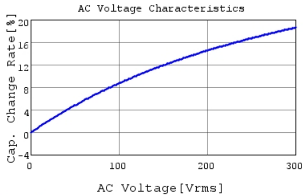
DE6B3KJ471KA3BE01J C-AC Voltage capchange, I
