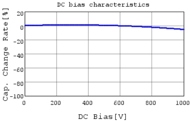
DE6B3KJ471KA4BE01J C-DC bias capchange, 20.0
