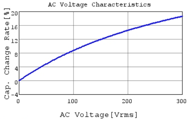
DE6B3KJ471KA4BE01J C-AC Voltage capchange, I
