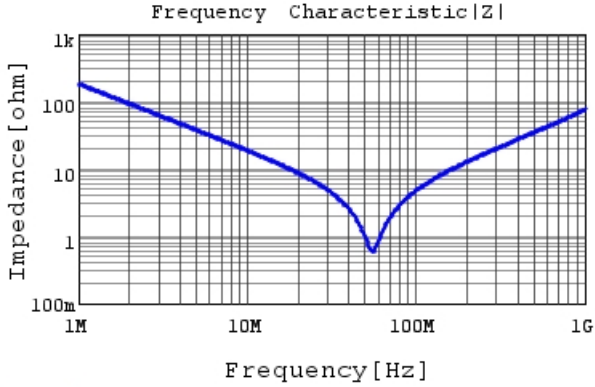
DE6E3KJ102MN4A |Z| DCOV, 20degC
