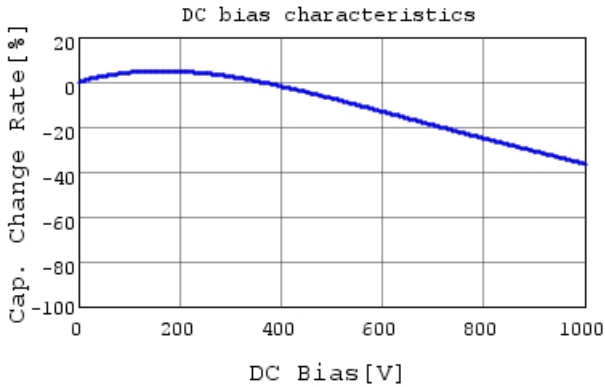
DE6E3KJ102MN4A C-DC bias capchange, 20.0degC
