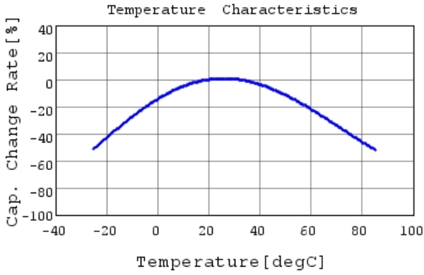
DE6E3KJ102MN4A C-Temp. capchange, DCOV, AC1V
