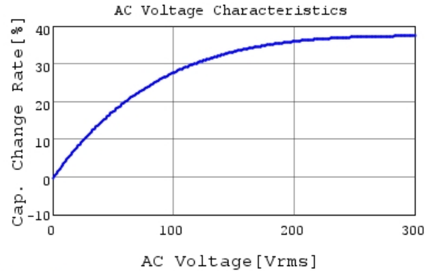
DE6E3KJ102MN4A C-AC Voltage capchange, DCOV,
