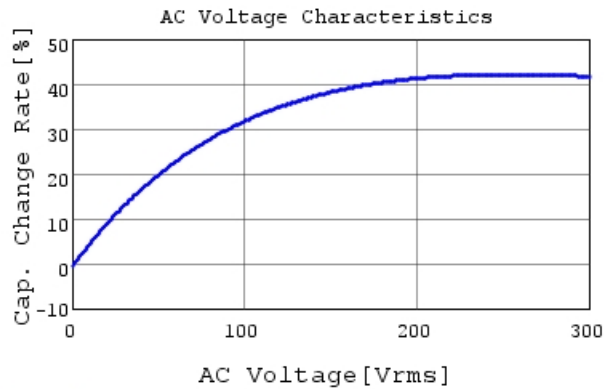
DE6E3KJ472MA4B C-AC Voltage capchange, DC0V,
