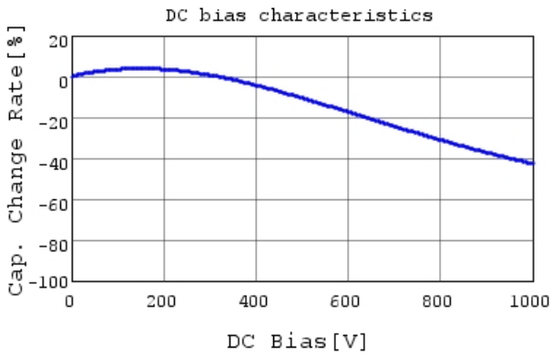
DE6E3KJ472MA4B C-DC bias capchange, 20.0degC
